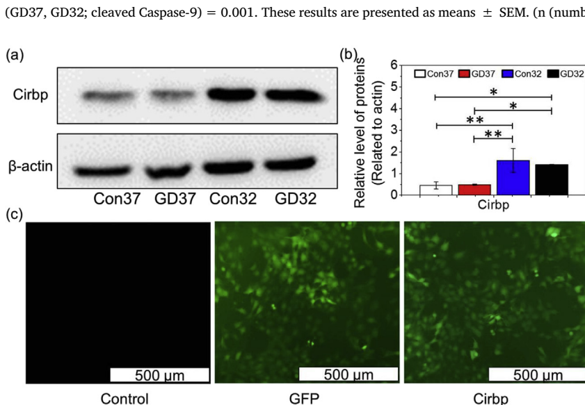
Fig. 5. Cirbp was upregulated under hypothermic conditions. (a) Cirbp was detected by western blot. \beta -actin was used as a loading control protein. (b) Protein bands on the western blots were scanned, and the intensity was determined by optical density measurements. The molecular weight of Cirbp and \beta -actin are 19 and 43 kD, respectively. F = 8.727. P (Con37, Con32) = 0.004. P (Con37, GD32) = 0.011. P (GD37, Con32) = 0.005. P (GD37, GD32) < 0.001. (c) 661w cells were transfected by GFP lentivirus and Cirbp lentivirus. These results are presented as means \pm SEM. (n (number of independent experiments) = 3. *: P < 0.05 , **: P < 0.01 ). Control: no vector control, GFP: Lenti-GFP transduction control, Cirbp: Lenti-Cirbp transduction group.
