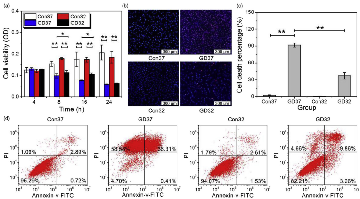
Fig. 1. Hypothermia treatment abrogates GD-injured cell death. (a) The 661 W cells were cultured in glucose-free medium for indicated times at 37 °C or 32 °C by MTT assay. F(8\text{ h}) = 82.926 . P(\text{Con37, GD37}; 8\text{ h}) < 0.001 . P(\text{Con32, GD32}; 8\text{ h}) < 0.001 . P(\text{GD37, GD32}; 8\text{ h}) = 0.019 . F(16\text{ h}) = 36.717 . P(\text{Con37, GD37}; 16\text{ h}) < 0.001 . P(\text{Con32, GD32}; 16\text{ h}) < 0.001 . P(\text{GD37, GD32}; 16\text{ h}) = 0.022 . F(24\text{ h}) = 63.202 . P(\text{Con37, GD37}; 24\text{ h}) < 0.001 . P(\text{Con32, GD32}; 24\text{ h}) < 0.001 . (b) The 661 W cells were cultured in glucose-free medium for 16 h at 37 °C or 32 °C by PI/Hoechst staining. (c) Quantitative assessment of cell death was performed with flow cytometry for PI/Hoechst staining. F = 301.908 . P(\text{Con37, GD37}) < 0.001 . P(\text{GD37, GD32}) < 0.001 . (d) Data from flow cytometry; 661w cells were stained by Annexin V-FITC and PI staining. Data are shown as means \pm SEM. n (number of independent experiments) = 3. *: P < 0.05 , **: P < 0.01 .
