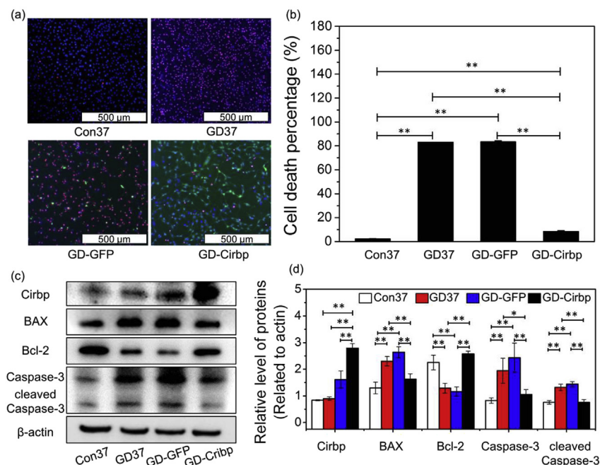
Fig. 6. Effects of overexpressing Cirbp in 661 W cells using Lenti-Cirbp. (a) The 661 W cells, GFP-lentivirus-transfected cells, and Cirbp-lentivirus-transfected cells were cultured in glucose-free medium for 16 h at 37 °C by PI/Hoechst staining. (b) Quantitative assessment of cell death was performed with flow cytometry for PI/Hoechst staining. F = 7549.26. P (Con37, GD37) < 0.001. P (Con37, GD-GFP) < 0.001. P (Con37, GD-Cirbp) < 0.001. P (GD37, GD-Cirbp) < 0.001. P (GD-GFP, GD-Cirbp; Cirbp) < 0.001. F (BAX) = 18.598. P (Con37, GD37; BAX) = 0.001. P (Con37, GD-GFP; BAX) < 0.001. P (GD37, GD-Cirbp; BAX) < 0.001. P (GD-GFP, GD-Cirbp; BAX) < 0.001. F (Caspase-3) = 12.13. P (Con37, GD37; Caspase-3) = 0.007. P (Con37, GD-GFP; Caspase-3) = 0.001. P (GD37, GD-Cirbp; Caspase-3) = 0.2. P (GD-GFP, GD-Cirbp; Caspase-3) = 0.002. F (cleaved Caspase-3) = 40.628. P (Con37, GD37; cleaved Caspase-3) < 0.001. P (Con37, GD-GFP; cleaved Caspase-3) < 0.001. P (GD37, GD-Cirbp; cleaved Caspase-3) < 0.001. P (GD-GFP, GD-Cirbp; cleaved Caspase-3) < 0.001. These results are presented as means \pm SEM. (n (number of independent experiments) = 3. *: P < 0.05 , **: P < 0.01 ). Con: no vector control, GFP: Lenti-GFP transduction control, Cirbp: Lenti-Cirbp transduction group.
