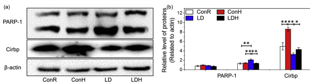
Fig. 9. Hypothermia treatment suppresses PARP-dependent apoptotic pathway. (a) PARP-1 and Cirbp were detected by western blot. \beta -actin was used as a loading control protein. The molecular weight of PARP-1, Cirbp and \beta -actin are 116, 89, 19 and 43 kD, respectively. (b) Protein bands on the western blots were scanned, and the intensity was determined by optical density measurements. F(\text{PARP-1}) = 26.501 . P(\text{ConR, LD}; \text{PARP-1}) < 0.001 . P(\text{ConH, LD}; \text{PARP-1}) < 0.001 . P(\text{LD, LDH}; \text{PARP-1}) < 0.001 . F(\text{Cirbp}) = 64.5 . P(\text{ConR, LD}; \text{Cirbp}) < 0.001 . P(\text{ConH, LD}; \text{Cirbp}) < 0.001 . P(\text{LD, LDH}) = 0.033 . These results are presented as means \pm SEM. (n (number of independent experiments) = 3. *: P < 0.05 , **: P < 0.01 ).
