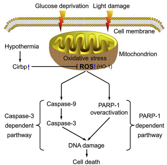
Scheme 1. A schematic diagram of the mechanism of hypothermia protective effect.
